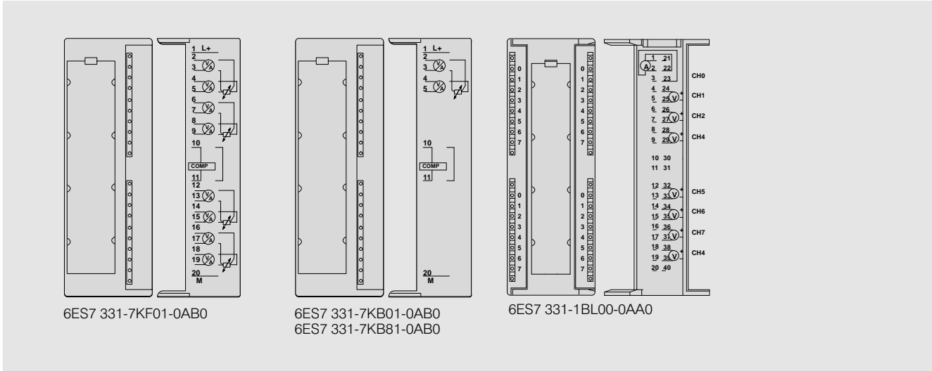
Fig. 1/10 Terminal connection diagram of the SM 331 analog input modules
