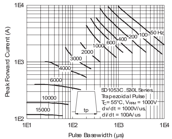
Fig. 39 - Frequency Characteristics
