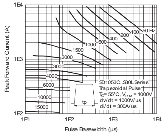
Fig. 37 - Frequency Characteristics
