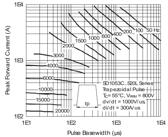
Fig. 31 - Frequency Characteristics
